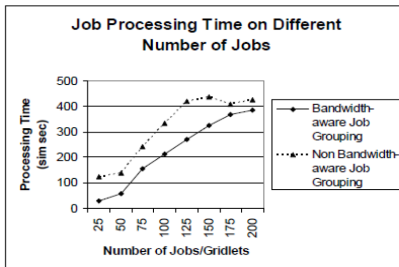
Fig. 4: Processing Time on Different Number of Jobs
