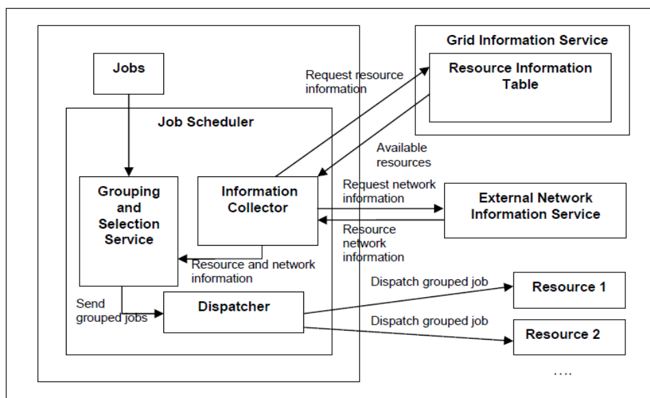
Fig. 1: Bandwidth-aware Job Grouping-based Scheduling Framework
