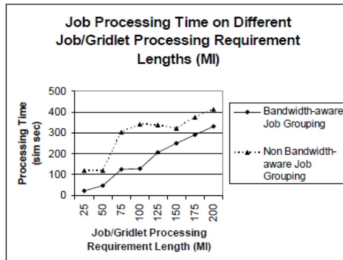
Fig. 5: Processing Time on Different Processing Requirement Lengths
