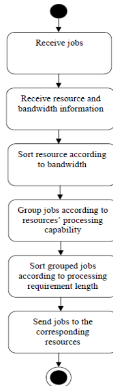
Fig. 3: Activity Diagram for Bandwidth-aware Job Grouping-based Scheduling Framework
